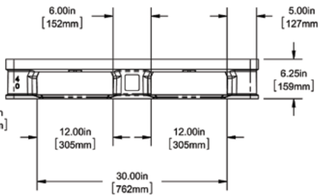
SIDE VIEW - 40"
