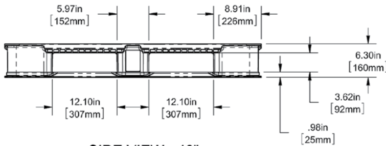
SIDE VIEW - 48"
