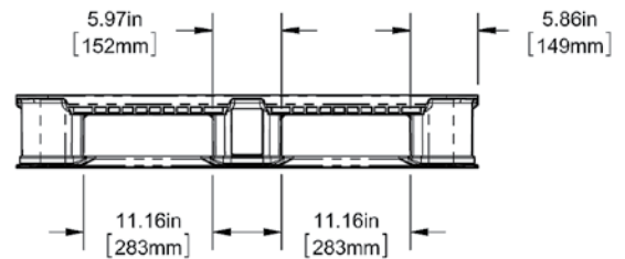
SIDE VIEW - 40"
